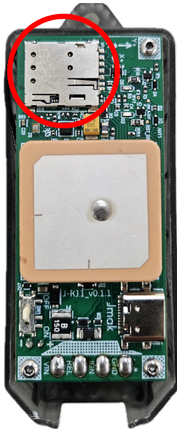
Figura 4: Simcard J-R11
